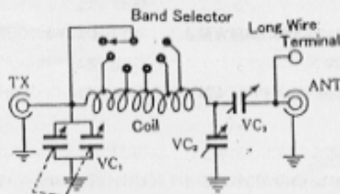
FIG. 1 CIRCUIT
